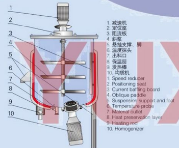
桨式搅拌 Paddle type blending
